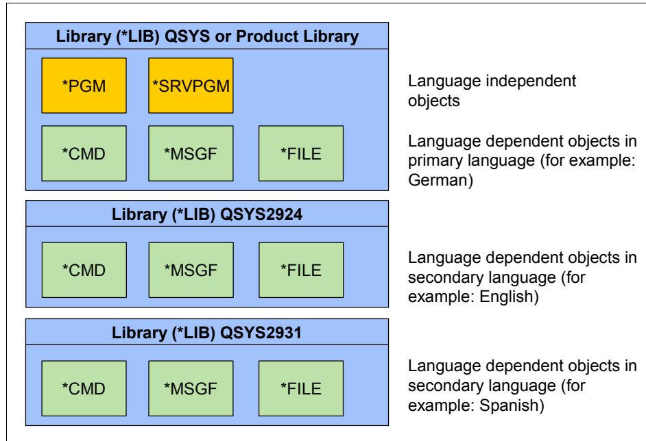
Figure 8-12 Object and file system language support
