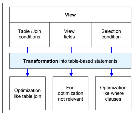
Figure 26-14 Use views to optimize a query
