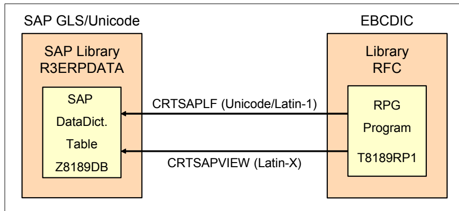
Figure 29-9 Accessing SAP dictionary tables from outside the SAP system
