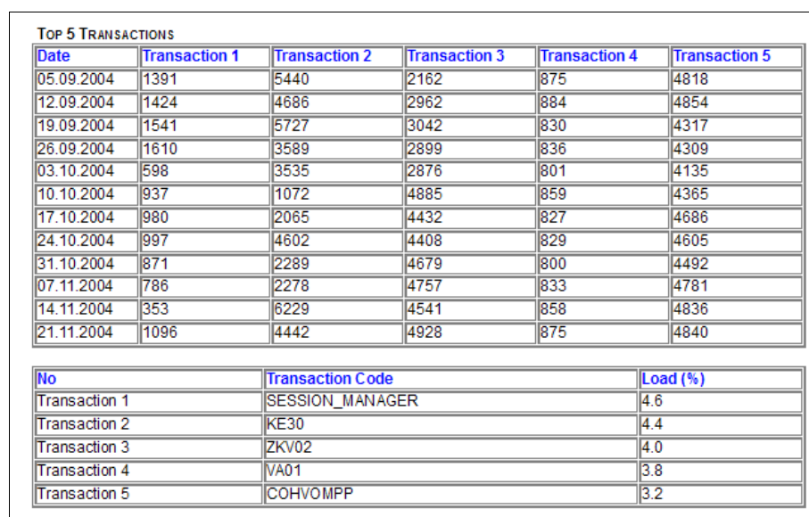
Figure 27-2 SAP EarlyWatch: trend of response time for the top five transactions
