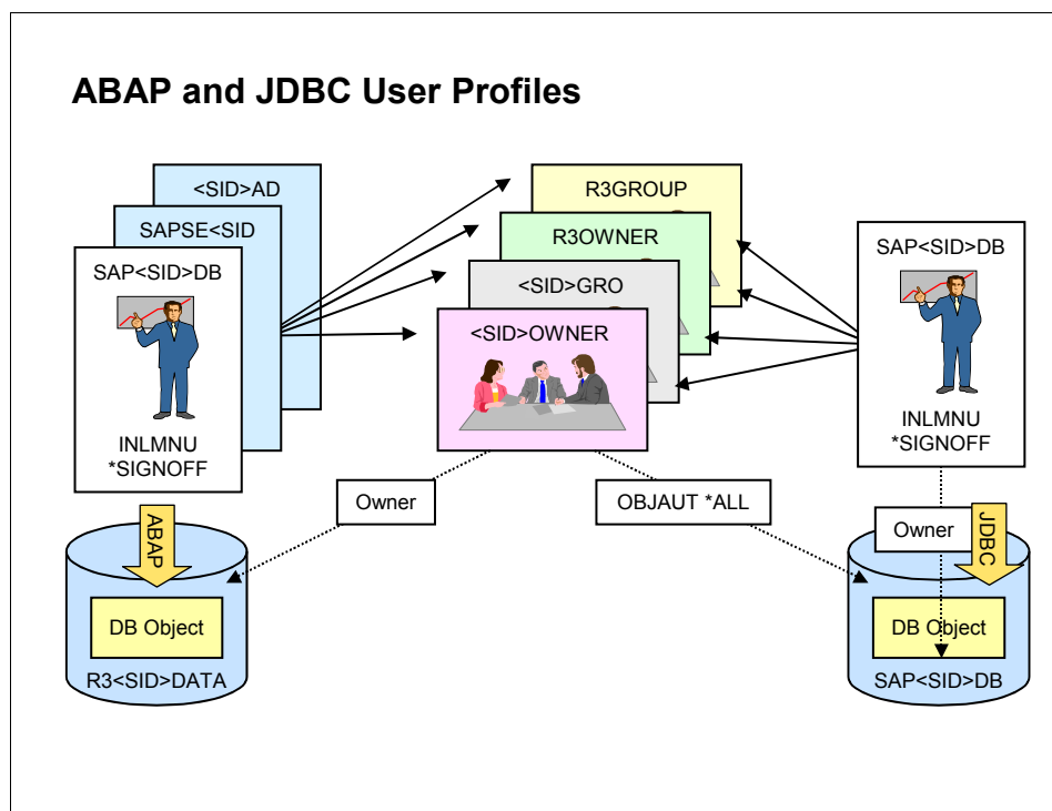
Figure 10-7 SAP ABAP and JDBC user profiles
