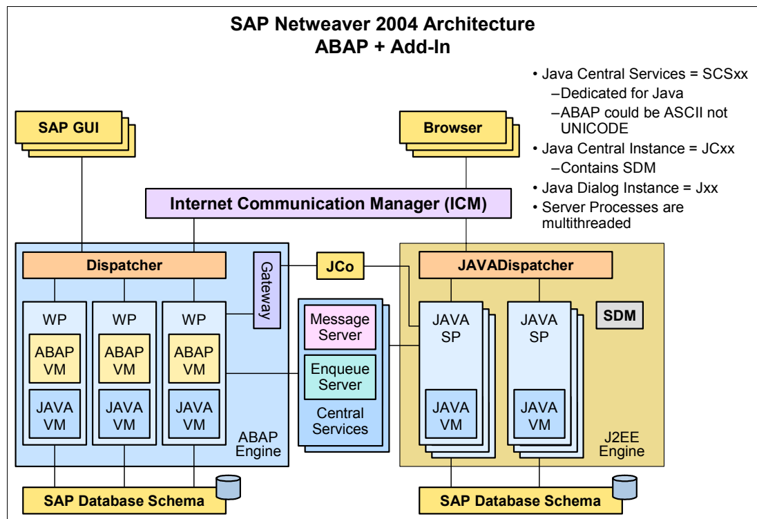
Figure 2-4 SAP NetWeaver Architecture, ABAP and Java
