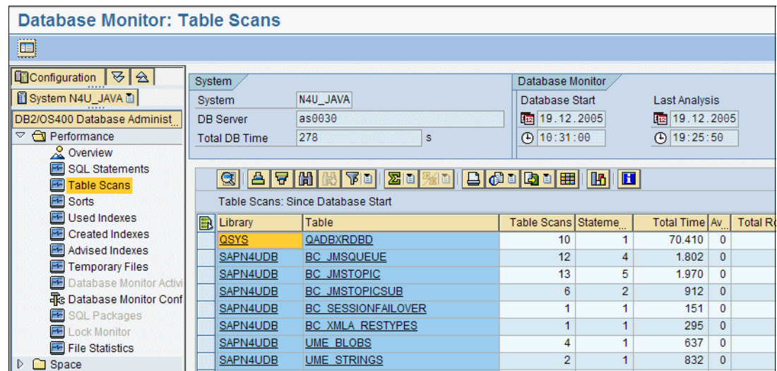
Figure 25-85 DB4COCKPIT - Table scans
