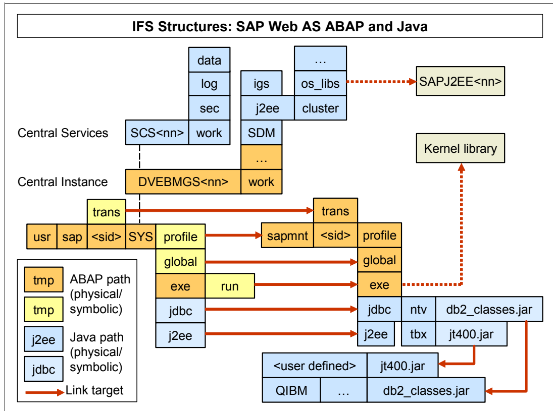
Figure 8-11 Integrated File System structures for the Web Application Server, ABAP and Java
