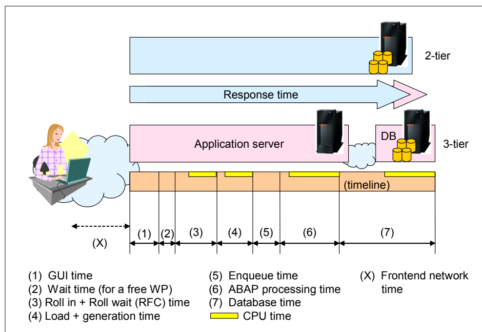
Figure 26-4 SAP system response time
