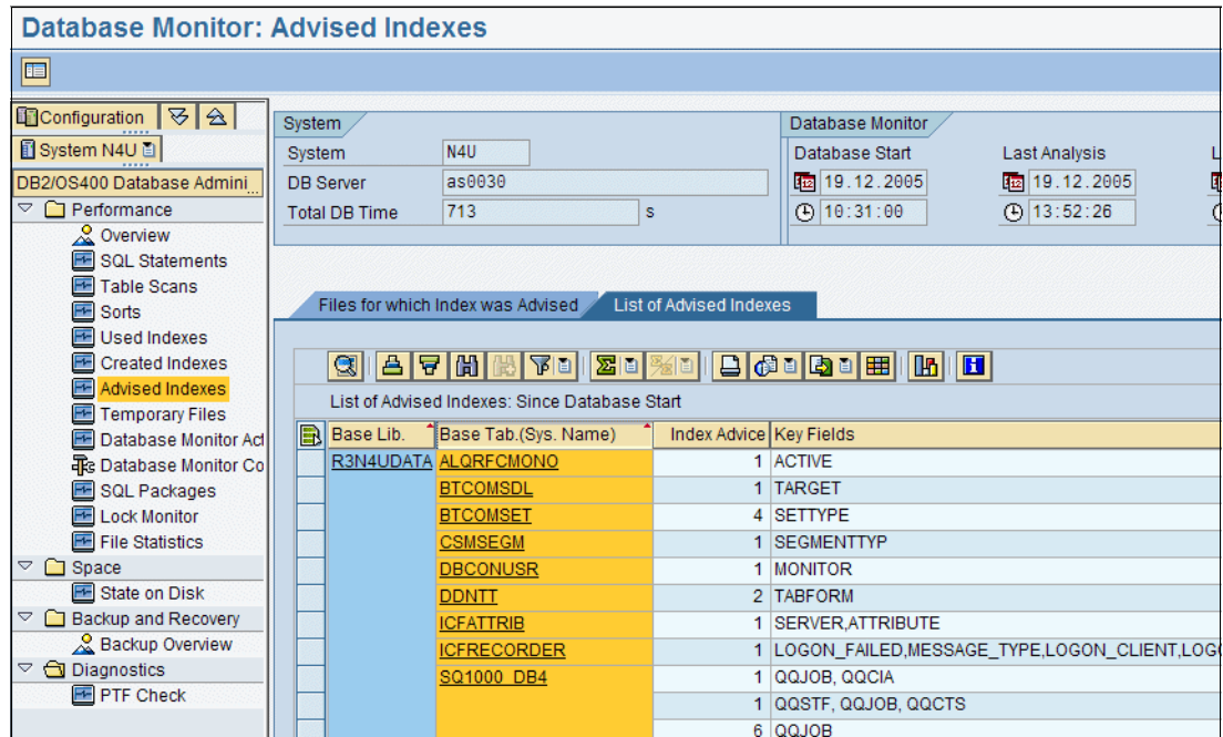
Figure 25-80 DB4COCKPIT - List of advised Indexes
