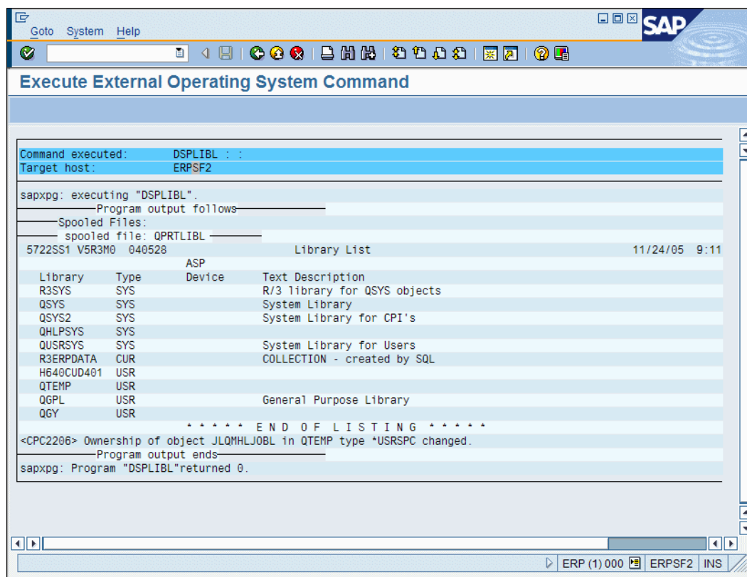
Figure 29-25 SAP program output results
