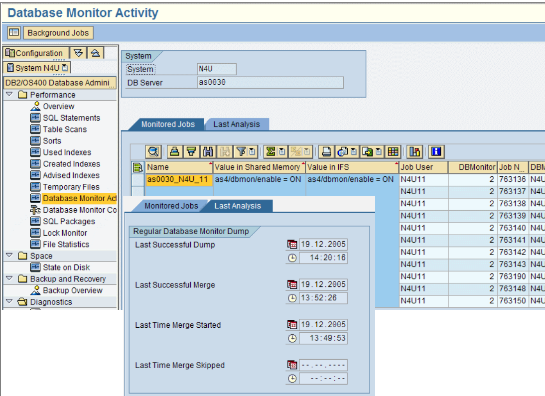
Figure 25-81 DB4COCKPIT - Database Monitor Activity - Monitored Jobs and Last Analysis
