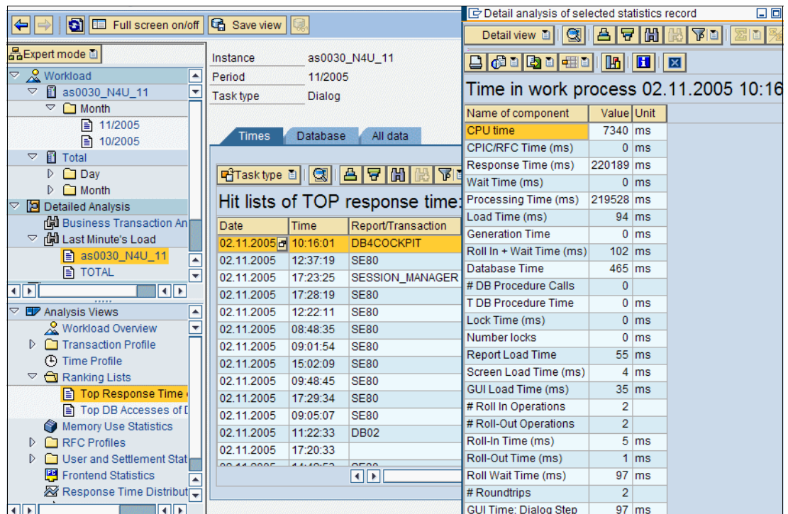
Figure 25-57 ST03 - top list of dialog transactions such as details for the first transaction
