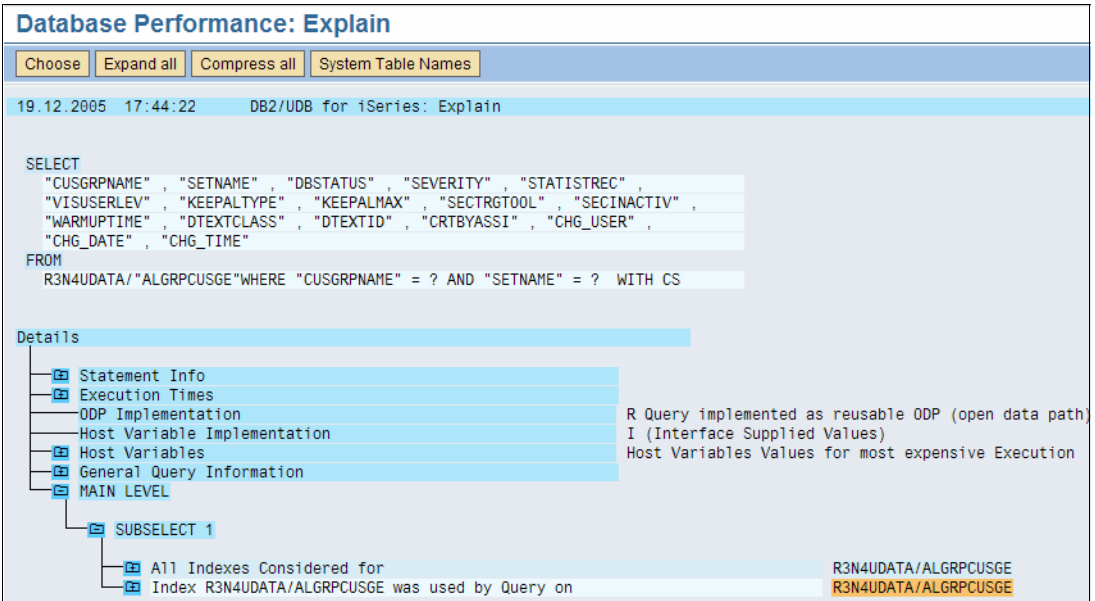
Figure 25-76 DB4COCKPIT - SQL statement detail
