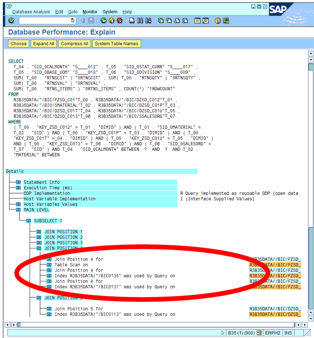
Figure 28-8 ST05 output for statement using LPG
