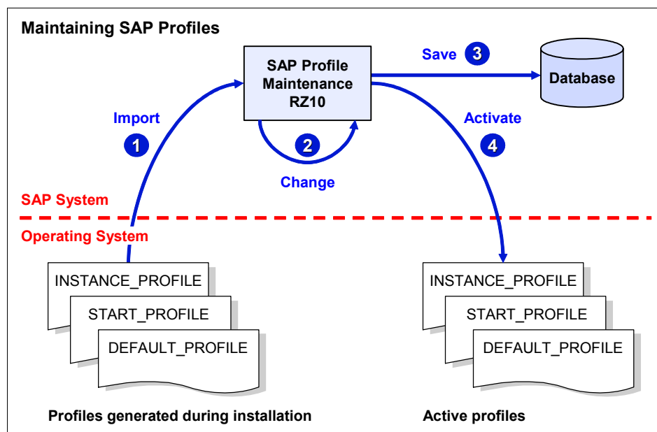
Figure 16-12 Maintaining SAP profiles
