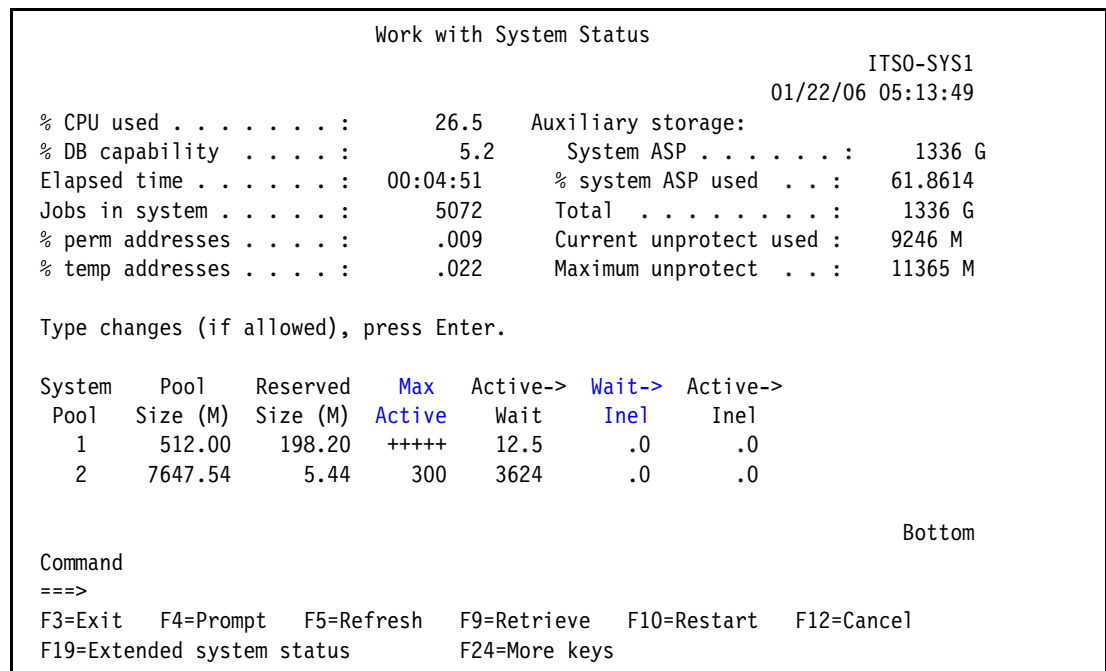
Figure 25-7 WRKSYSSTS (view 2) - F11 transition data
