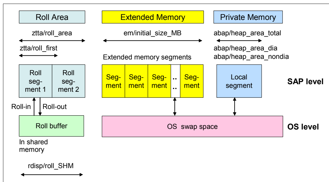
Figure 25-2 SAP memory management system
