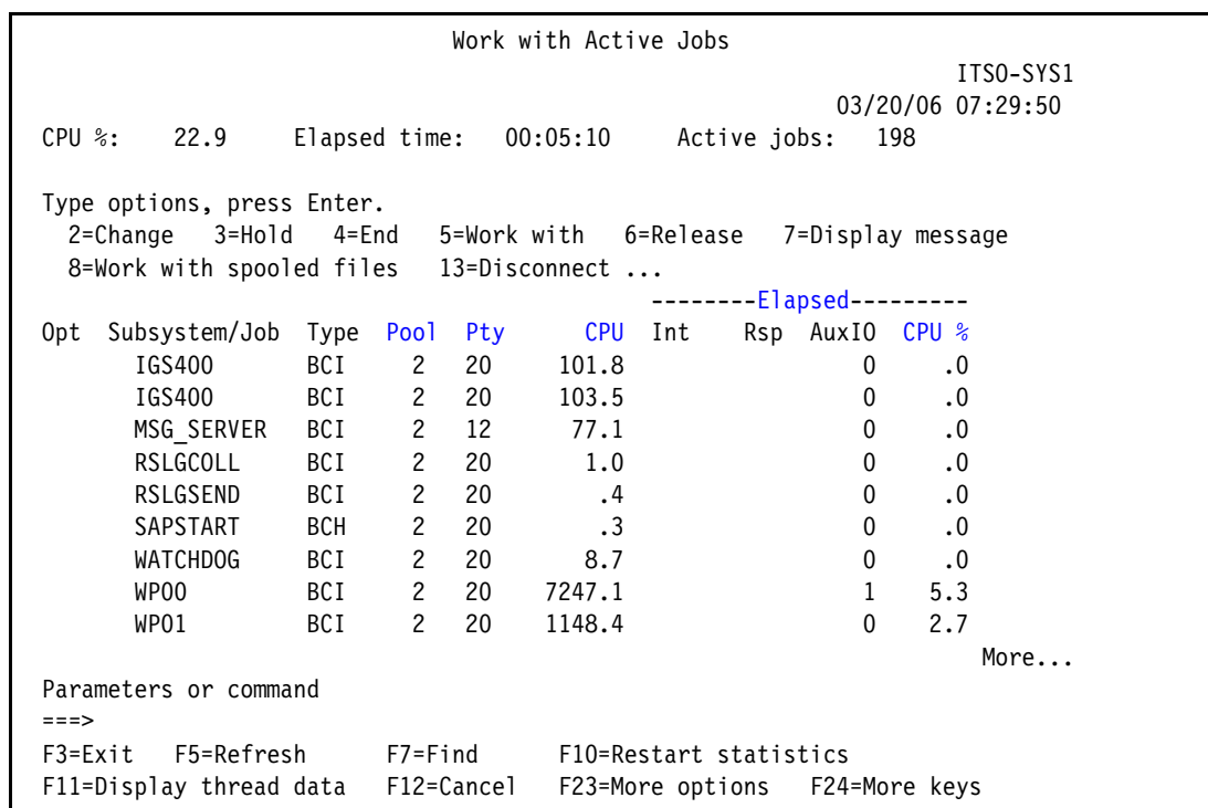
Figure 25-9 WRKACTJOB (view 1)
