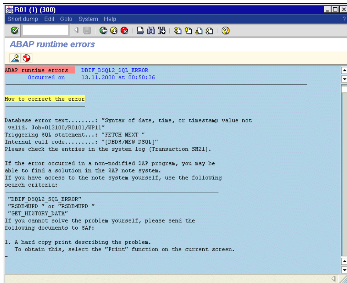
Figure 20-6 Short dump
