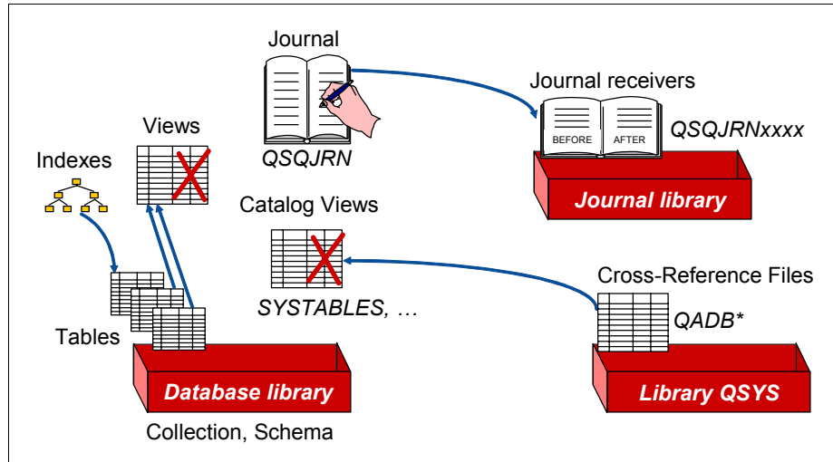
Figure 8-5 SQL collection
