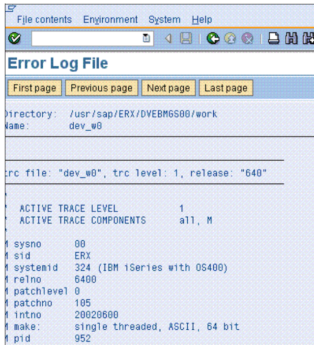
Figure 12-13 Extract from the developer trace
