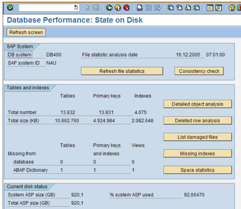
Figure 25-66 Database performance: State of Disk (ST02)
