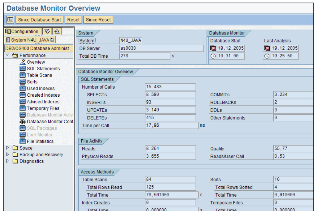
Figure 25-84 DB4COCKPIT - Database Monitor for the Java instance
