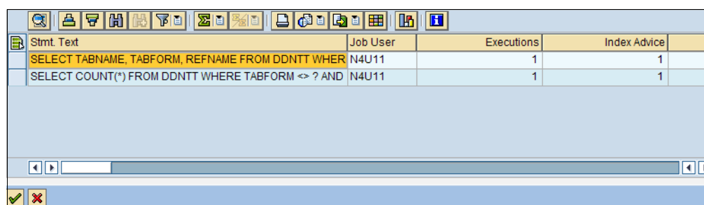
Figure 25-79 DB4COCKPIT - Advised Indexes - detail
