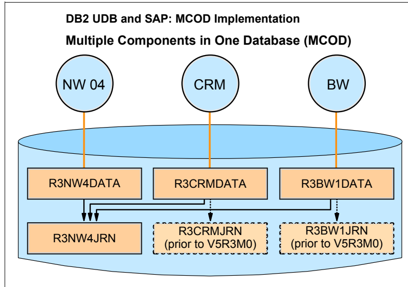
Figure 9-4 SAP databases in a MCODE implementation
