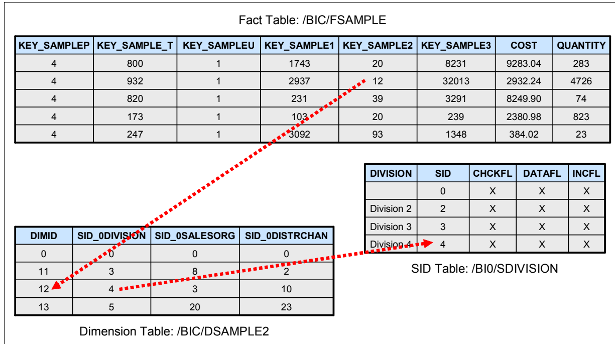
Figure 28-2 Use of surrogate keys in SAP BW
