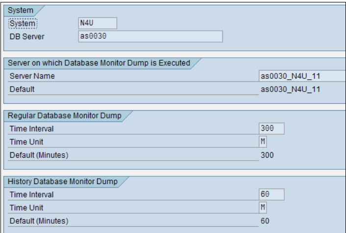
Figure 25-82 DB4COCKPIT - Database Monitor Configuration
