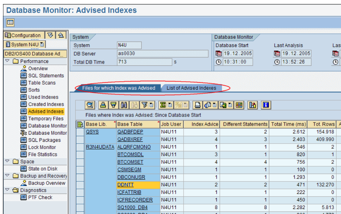
Figure 25-78 DB4COCKPIT - Advised Indexes
