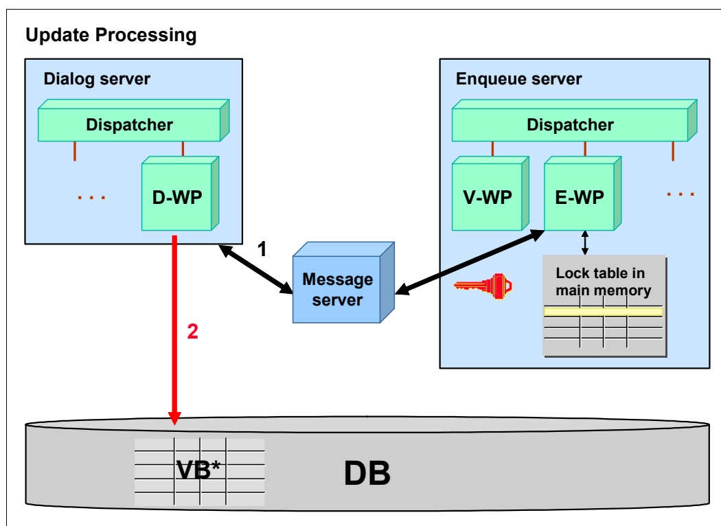
Figure 16-6 Update processing
