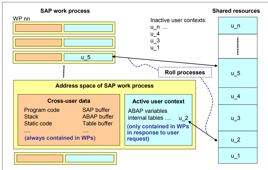
Figure 25-3 SAP work process and shared resources
