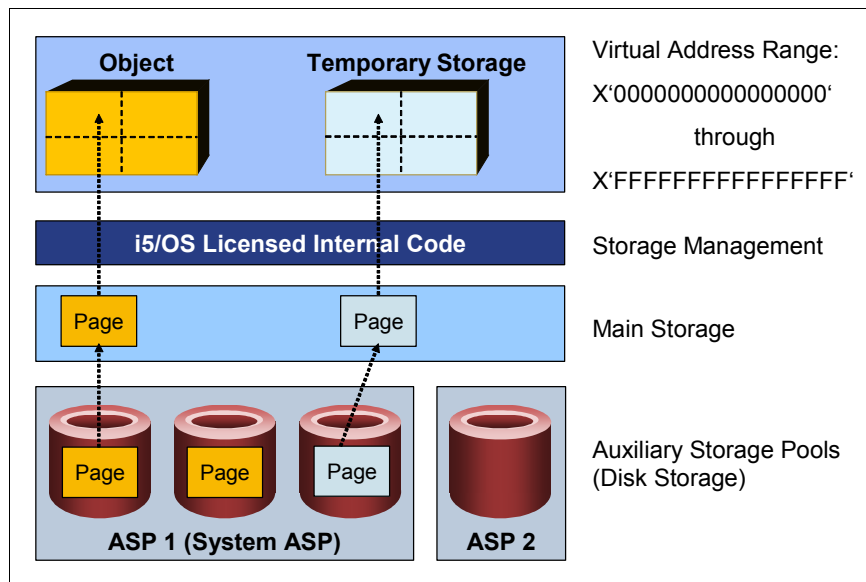
Figure 8-1 Single-level storage
