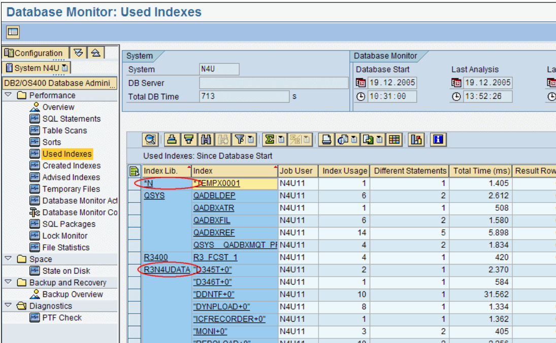
Figure 25-77 DB4COCKPIT - Used Indexes
