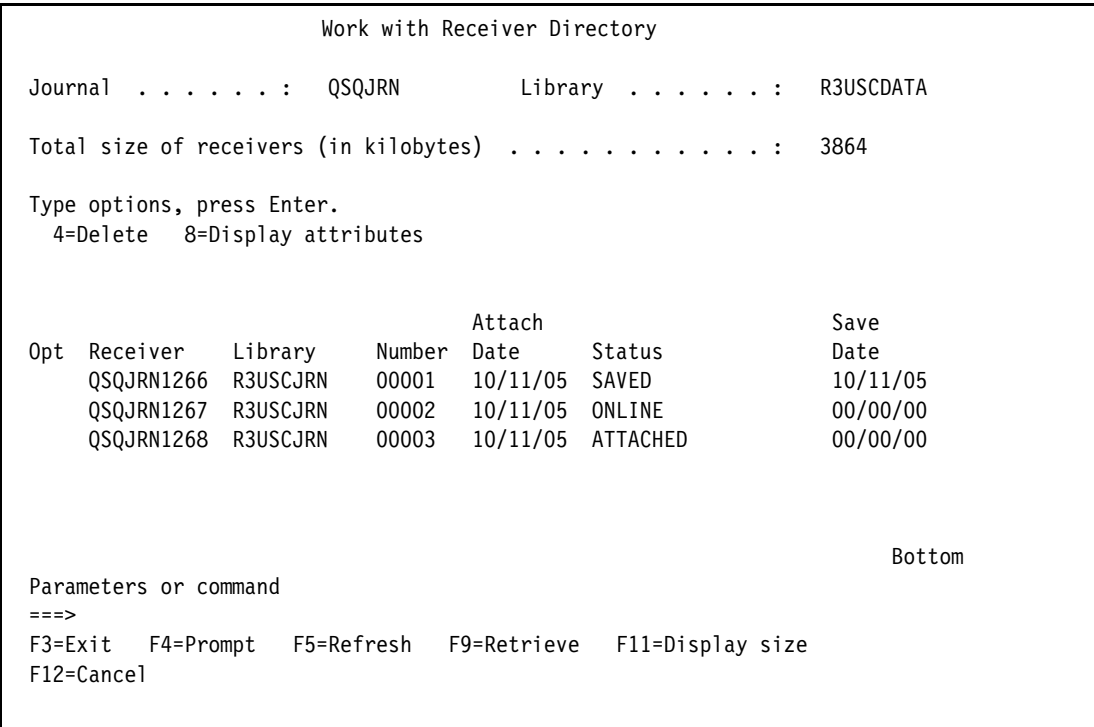
Figure 23-13 WRKJRNA and F15: work with receiver directory
