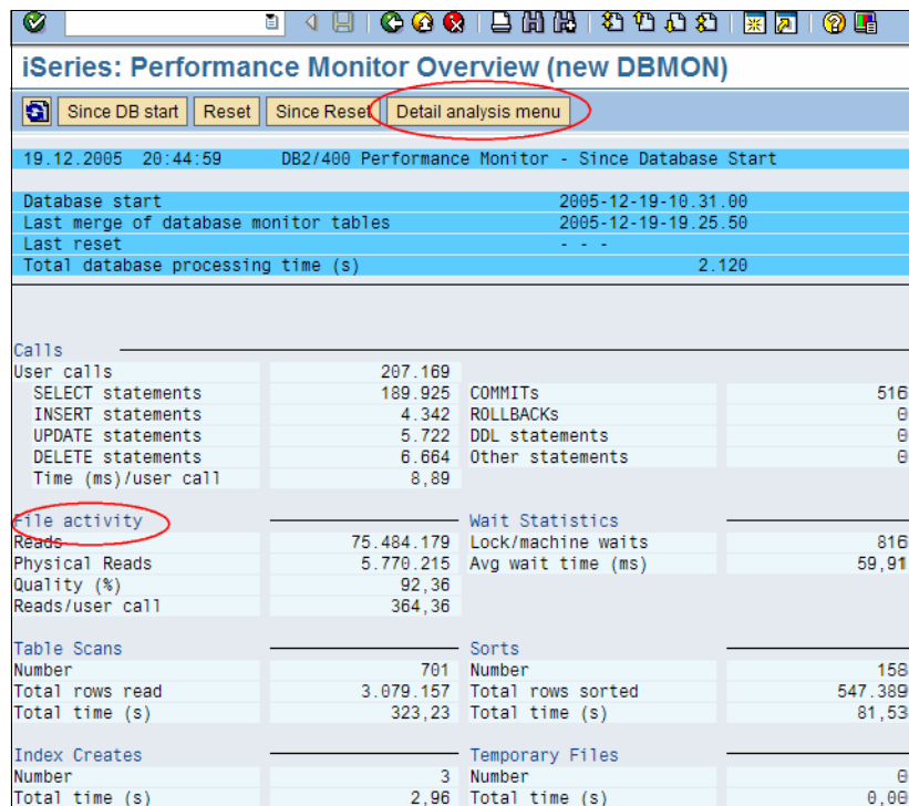
Figure 25-68 Database Performance Monitor (ST04)
