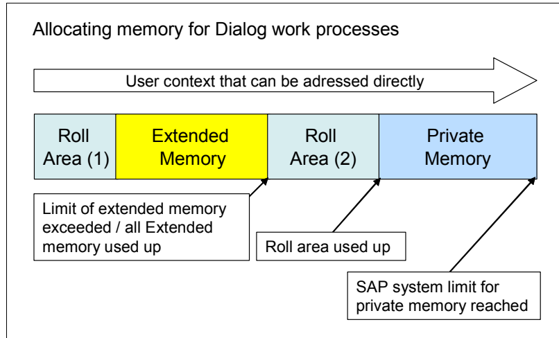
Figure 25-4 Allocation sequence for dialog work processes
