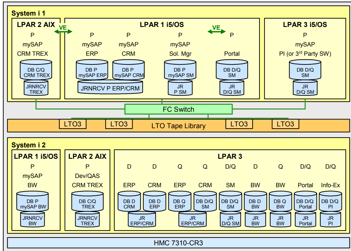
Figure 4-3 Large landscape example
