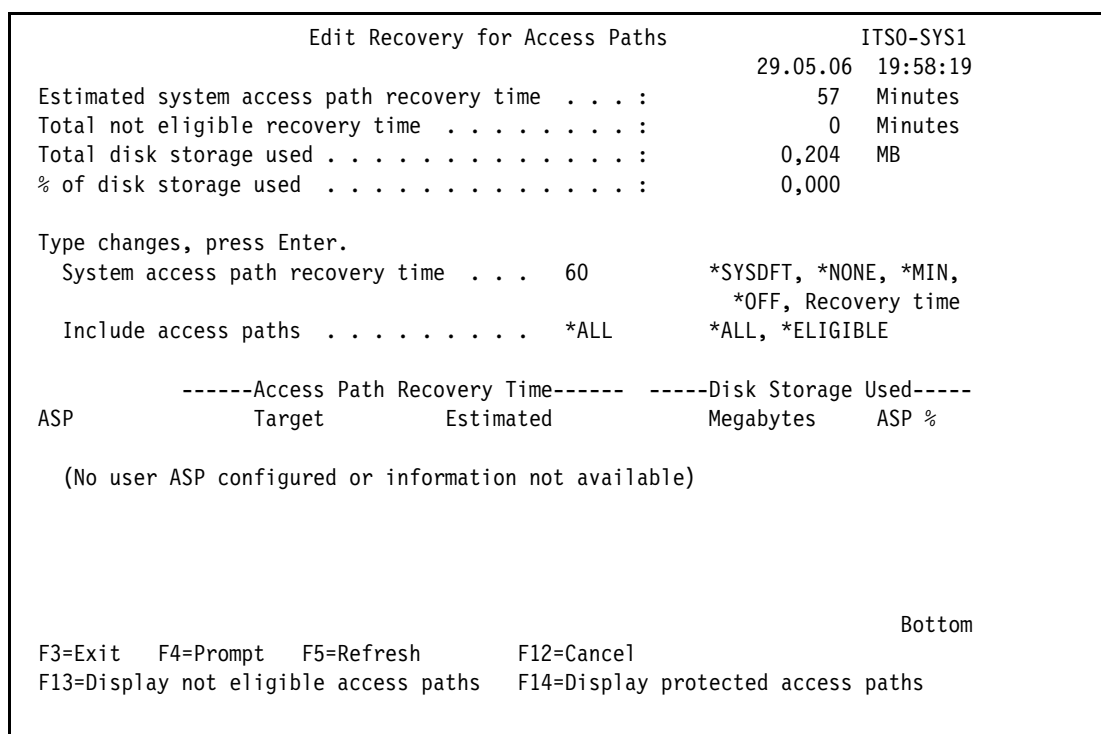
Figure 9-10 The i5/OS command EDTRCYAP (Edit Recovery for Access Paths)
