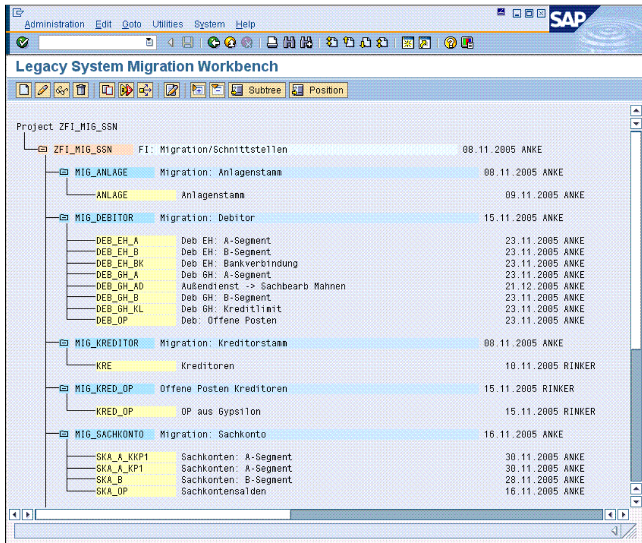
Figure 30-7 Project structure
